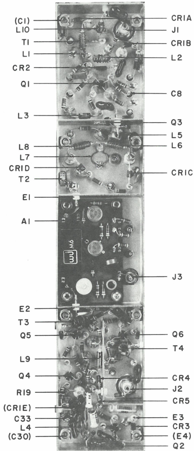
Figure 5-7. Type 71281 100-180 MHz Tuner (A1), Location of Components
