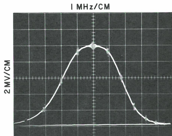
Figure 4-7. Typical 100-MHz RF Response Curve
