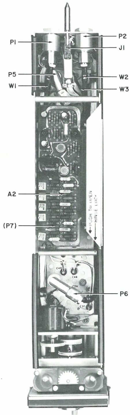
Figure 5-3. Type VH-13 Tuning Head, Top View, Location of Components
