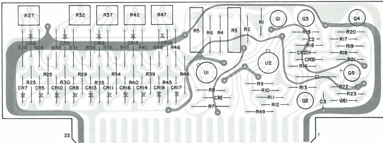
Figure 5-9. Type 79844-3 Shaping Amplifier (A2), Location of Components
