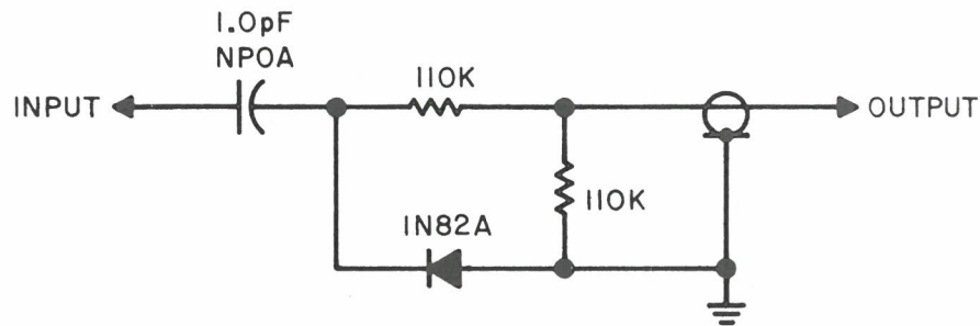
Figure 4-2. High Z Detector Diagram
