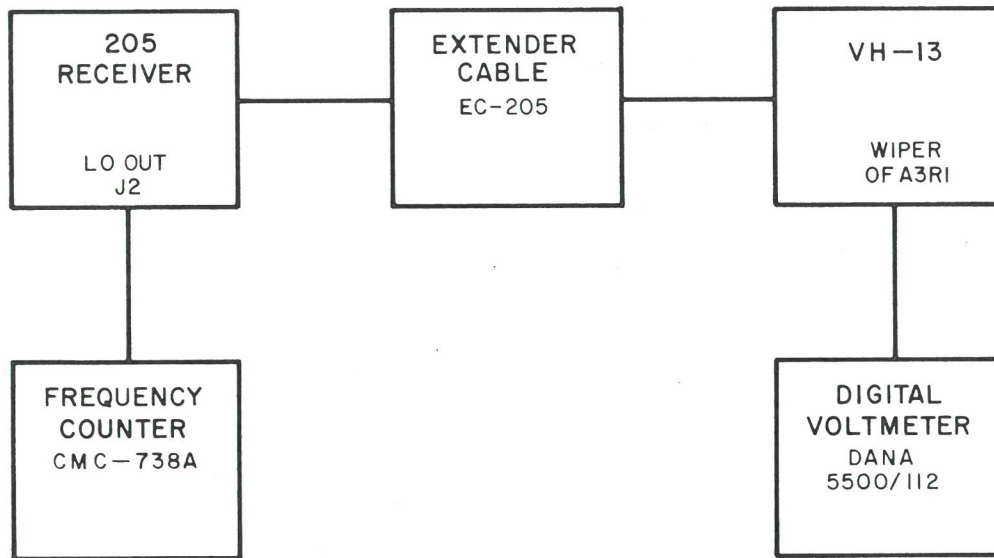
Figure 4-10. Test Equipment Connections, Shaping Amplifier Alignment
