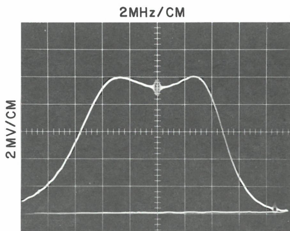
Figure 4-6. Typical 180-MHz RF Response Curve
