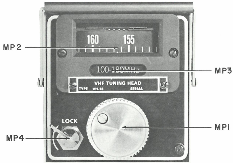
Figure 5-1. Type VH-13 Tuning Head, Front View, Location of Components
