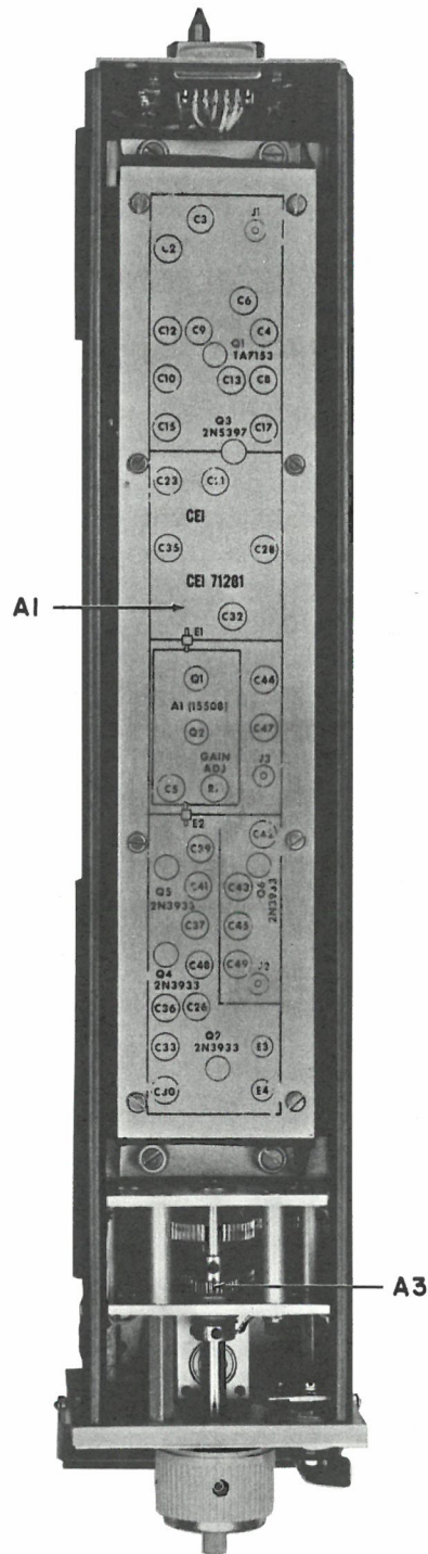
Figure 5-4. Type VH-13 Tuning Head, Bottom View, Location of Components
