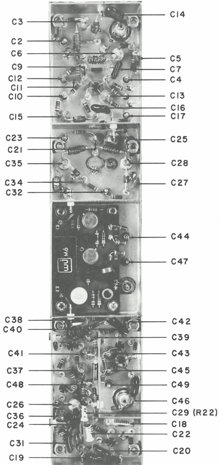
Figure 5-5. Type 71281 100-180 MHz Tuner (A1), Location of Components
