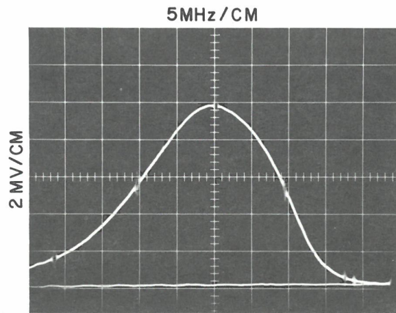
Figure 4-4. Typical 180 MHz RF Response Curve
