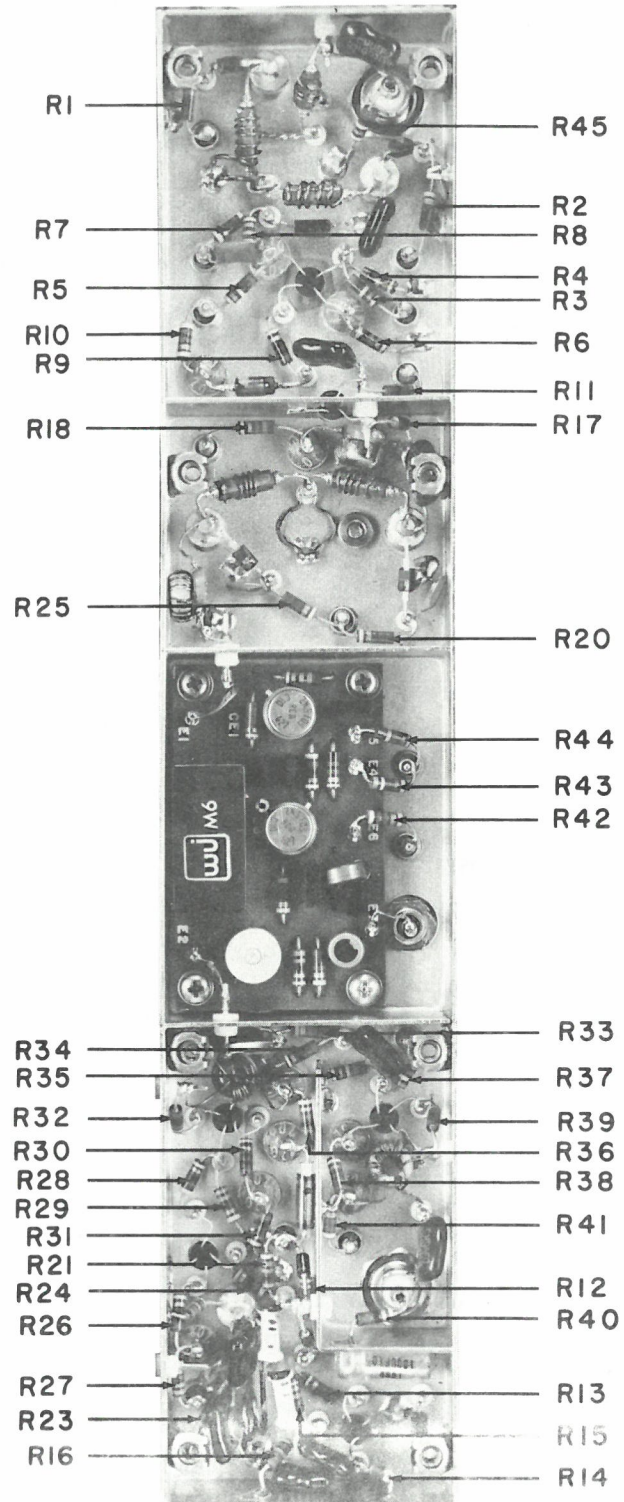
Figure 5-6. Type 71281 100-180 MHz Tuner (A1), Location of Components
