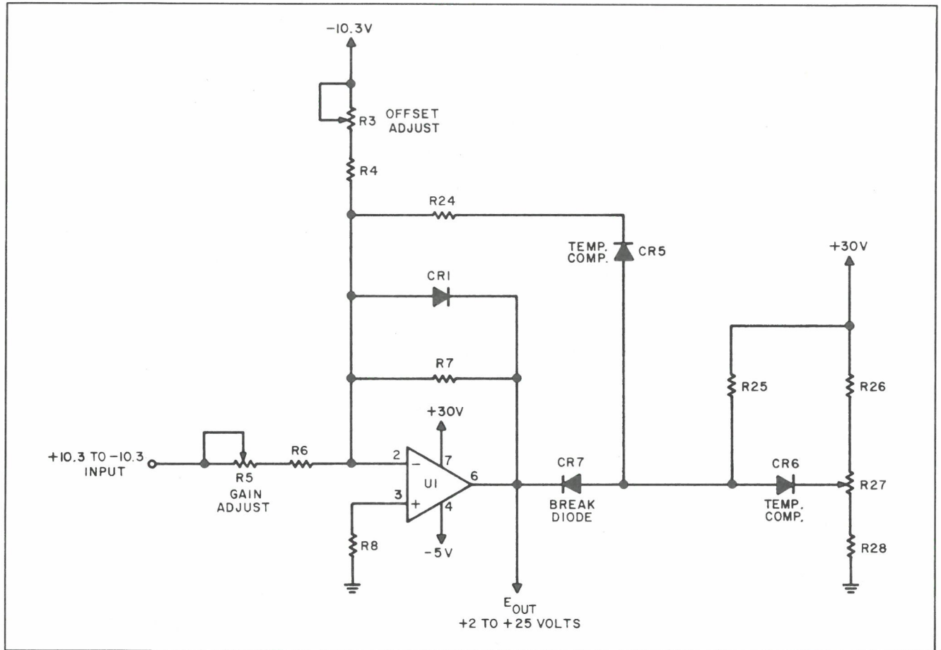
Figure 2-2. Shaping Amplifier, Simplified Diagram
