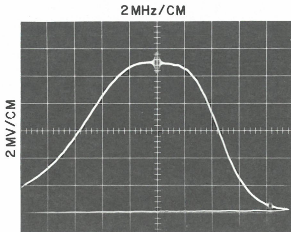
Figure 4-5. Typical 100-MHz RF Response Curve
