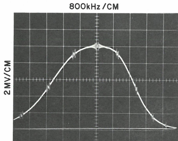
Figure 4-9. Typical IF Response Curve (100 MHz RF Input)
