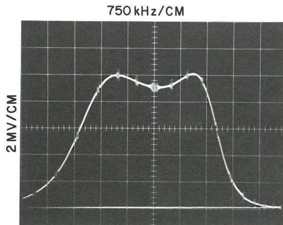
Figure 4-8. Typical IF Response Curve (180 MHz RF Input)
