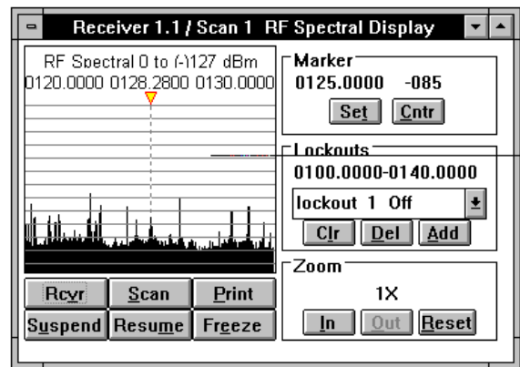
Figure 7. RF Spectral Display*
