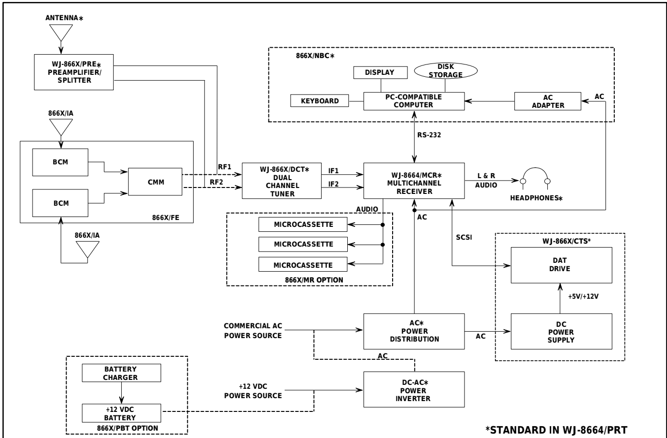
Figure 1. WJ-8664 System Block Diagram
