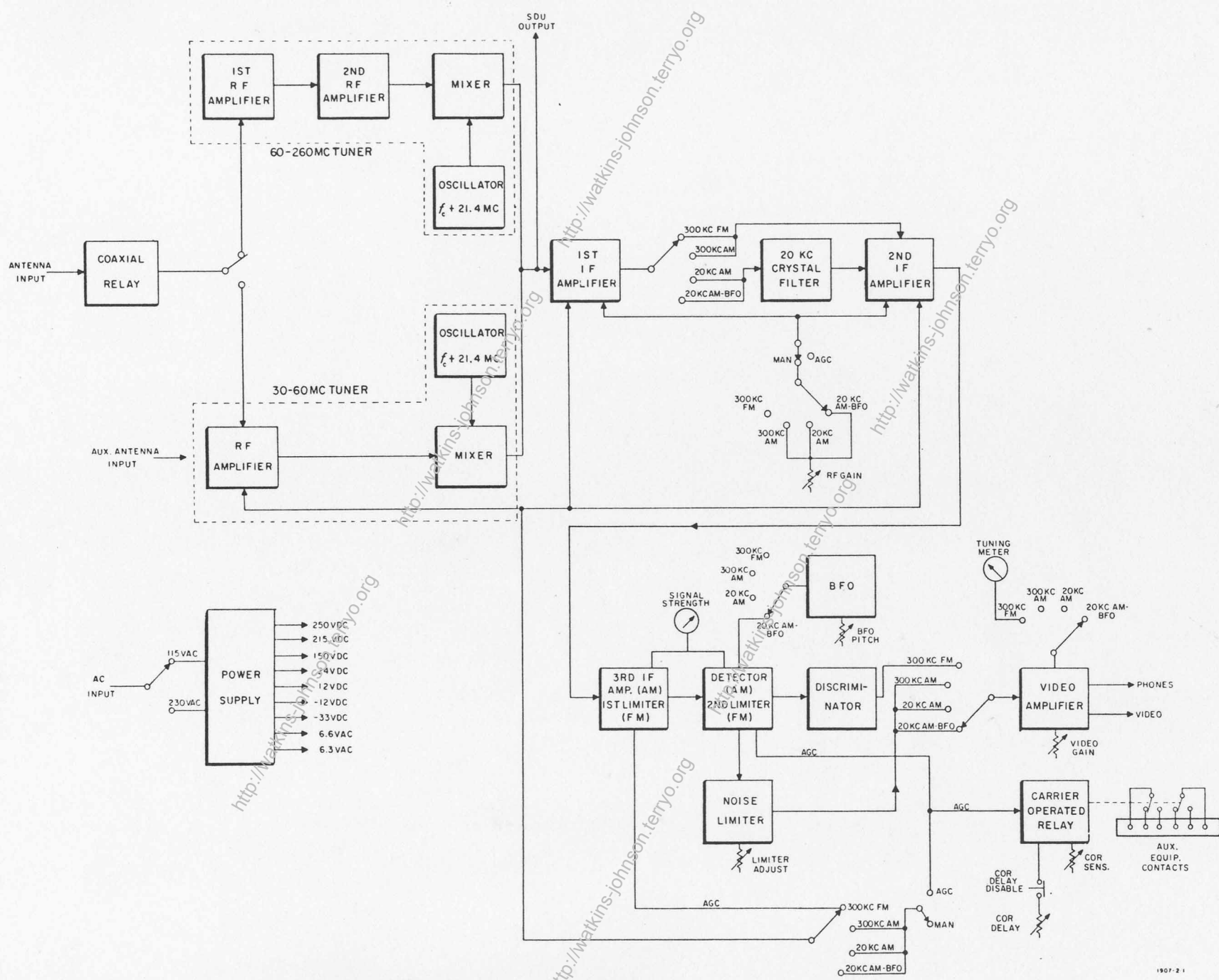
Figure 2-1. Block Diagram, Model 1907 Special Purpose Receiver
